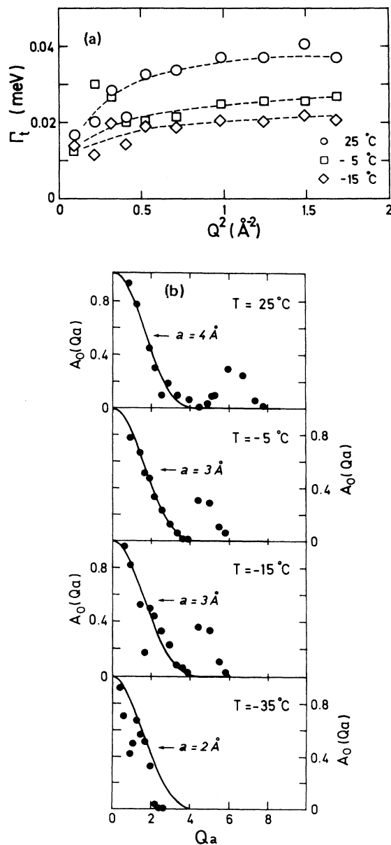
FIG. 9. (a) Restricted translational linewidth \Gamma_t of water contained in 25% hydrated Vycor plotted as a function of Q^2 at three temperatures: 25, -5, and -15 ^\circ\text{C} . (b) The elastic incoherent structure factor A_0(Qa) for water contained in 25% hydrated Vycor obtained from analysis of 9- \text{\AA} and 6- \text{\AA} data for four temperatures: 25, -5, -15, and -35 ^\circ\text{C} . Solid circles are the data and solid lines are the best fits using Eq. (19).
